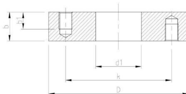
Double-sided tapped bulkhead flange
